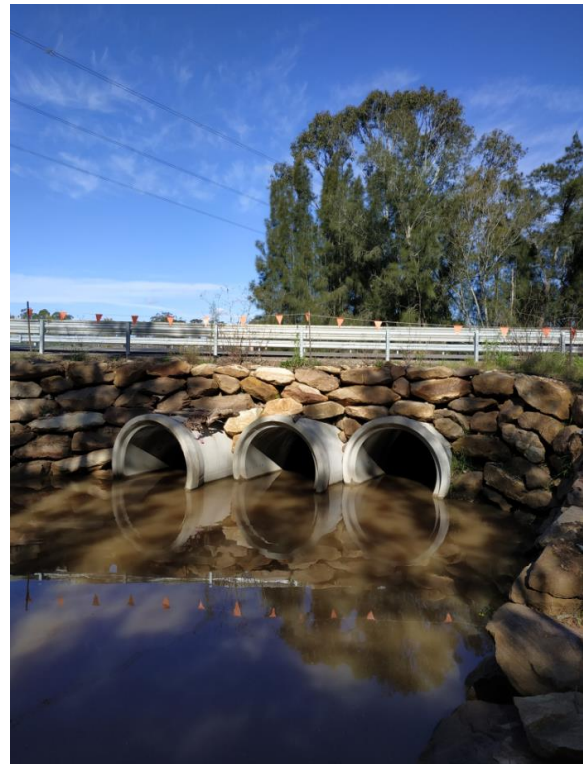
Photo 2 – 3x1.5m RCPs Paton Lane
